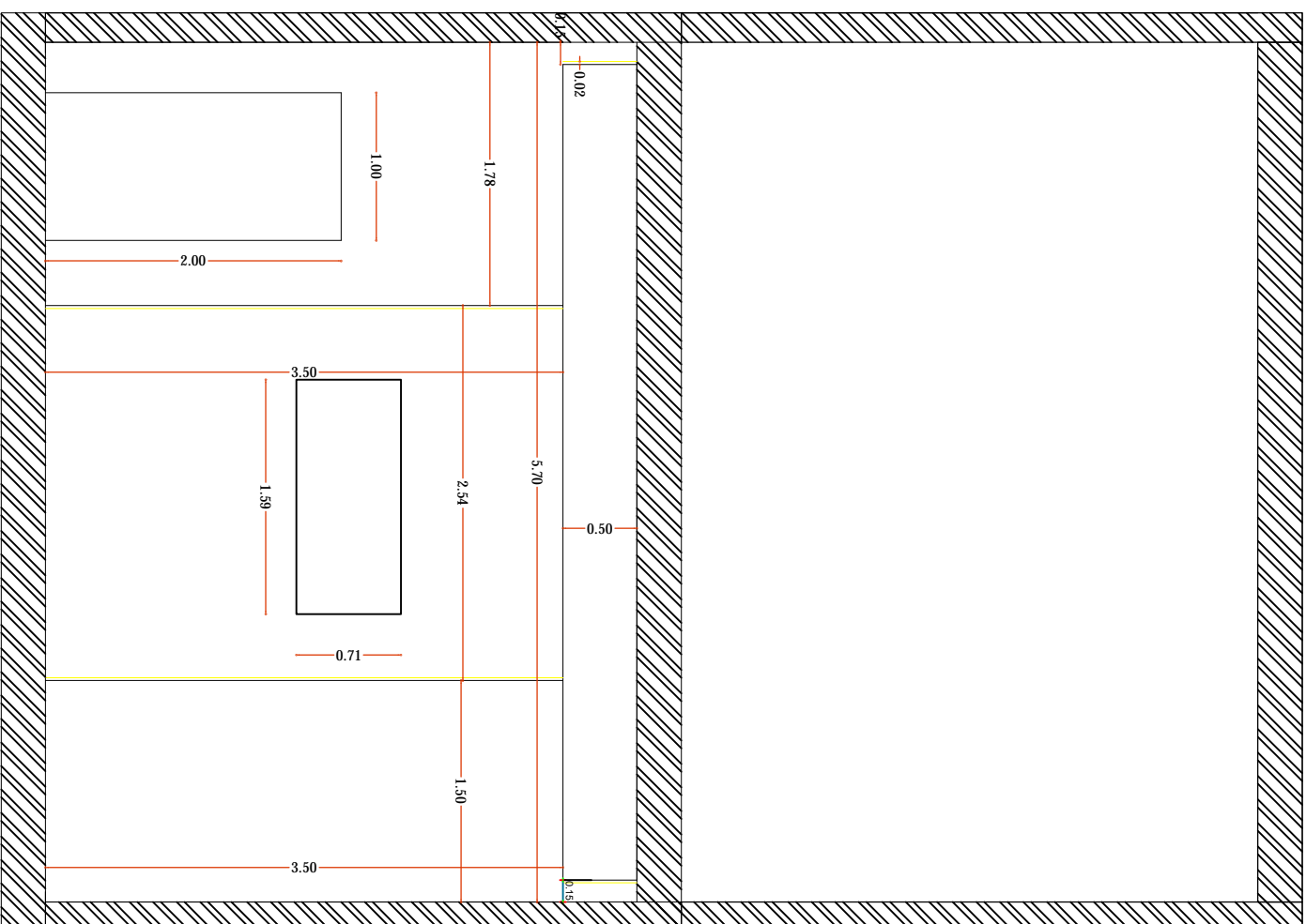
GROUND FLOOR 7 ELEVATION A (1) SCALE 1:50
